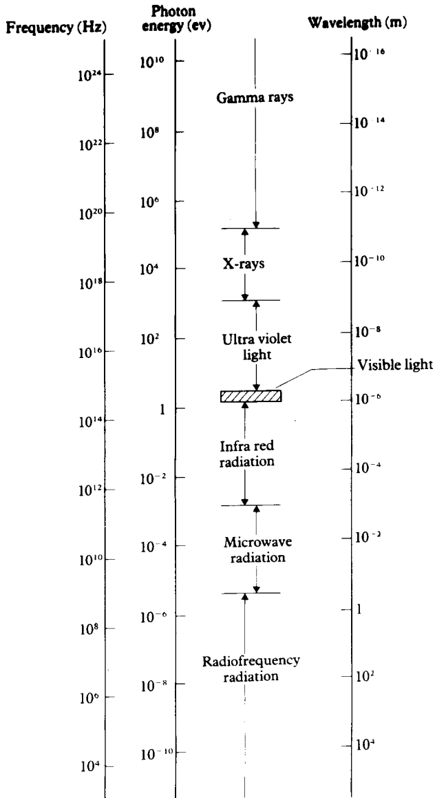
1.9 The electromagnetic spectrum.
